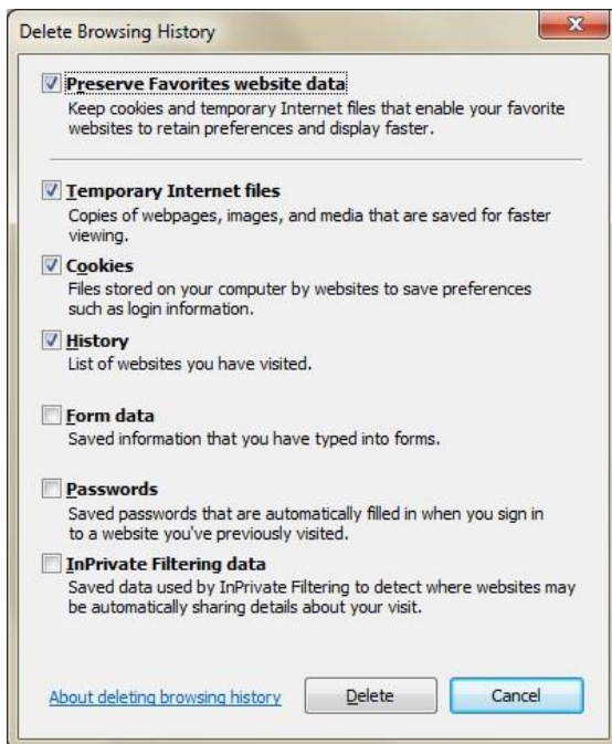
Figure 4: InPrivacy Browsing
